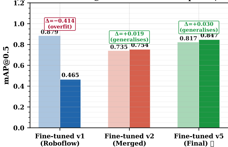
(a) Val vs Test mAP@0.5 Generalisation Gap — v1, v2, v5
